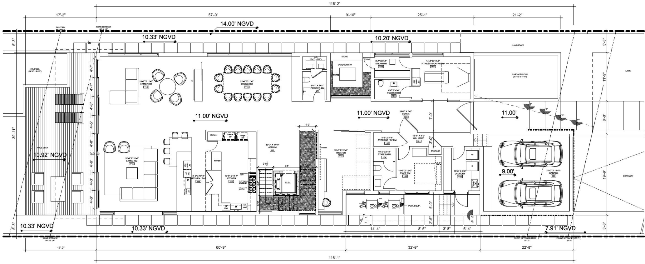
GROUND FLOOR
